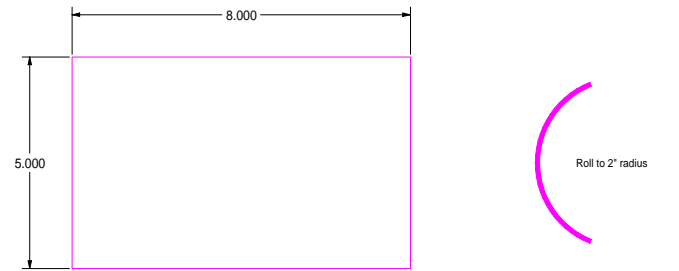
Baffle Plate 10 Ga Aluminum
